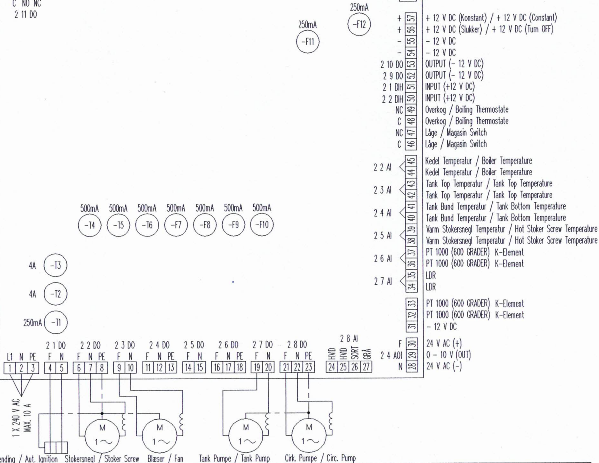
El-Tanding / Aut. Ignition Stokersnegl / Stoker Screw Blæser / Fan Tank Pumpe / Tank Pump Øirk. Pumpe / Circ. Pump
